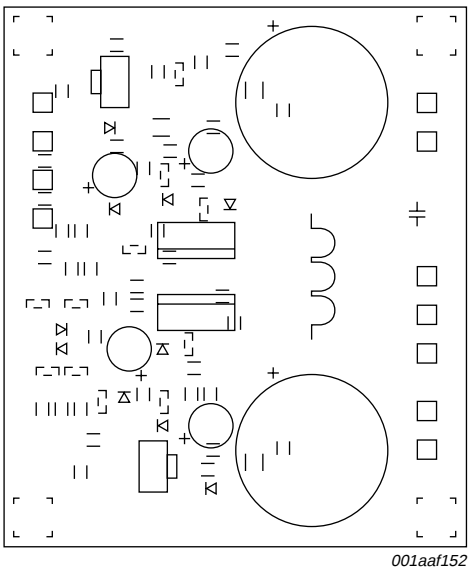
Fig 5. Component layout
