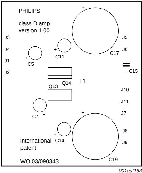
Fig 6. Top silk-screen
