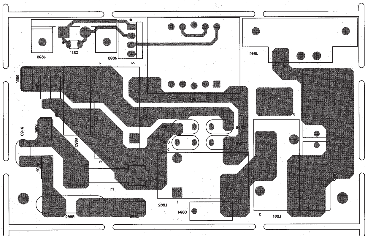
Solder Side
