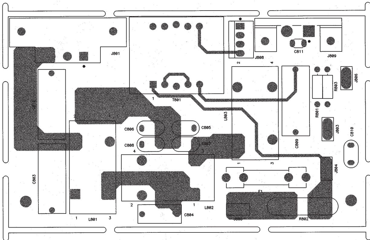
Component Side
