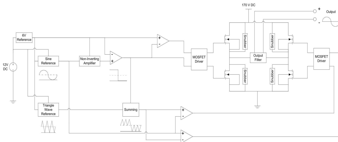
Figure 12: Block Diagram
