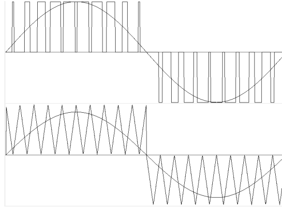
Figure 20: PWM Signal
