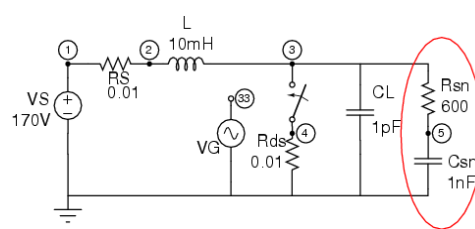
Figure 10: Inductive Load Circuit with Snubber
