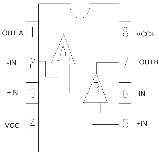
U102,103 104,105(TL072CP)
