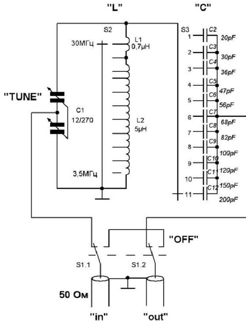
Figure 1 Pocket Antenna Tuner
