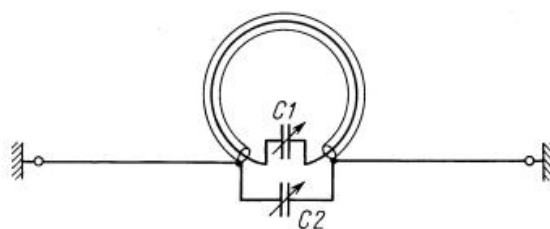
Figure 1 UA6AGW Antenna
