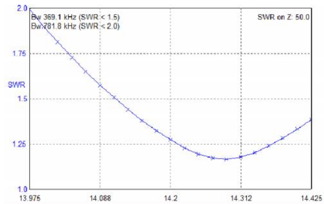
Figure 6 SWR of the Simple Folded Dipole Antenna in Free Space
