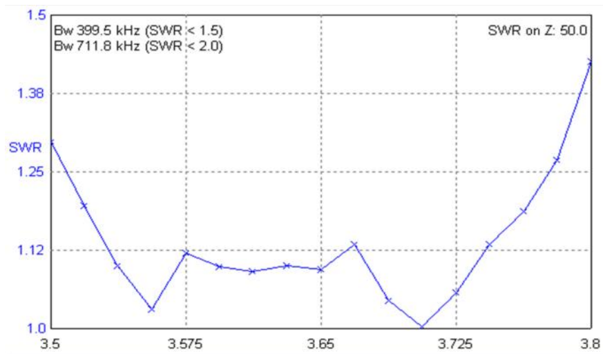
Figure 2 SWR of the Dipole Antenna for the 80- meters with rectangular UR0GT- Match (Installed at height of 30- m above the real ground)
