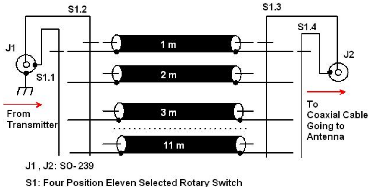
Figure 1 Simple HF ATU on lengths of Coaxial Cable
