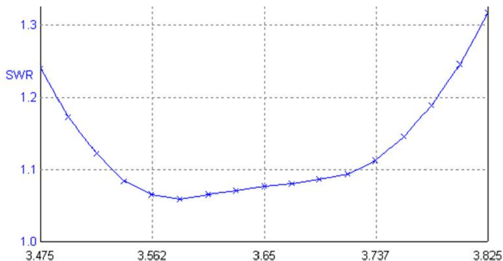
Figure 1 Design of the Narrow DEWD Dipole for the 80- meters with an Inductance Matching
