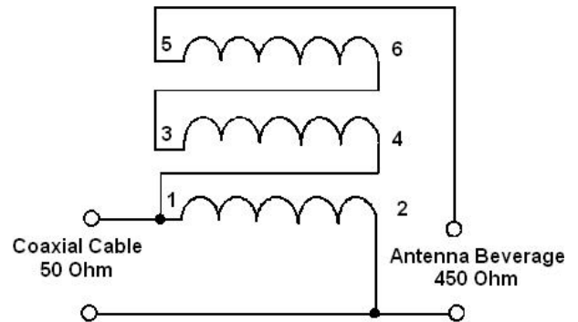
Figure 5 Schematic of Classical Unsymmetrical RF Transformer 1:9
