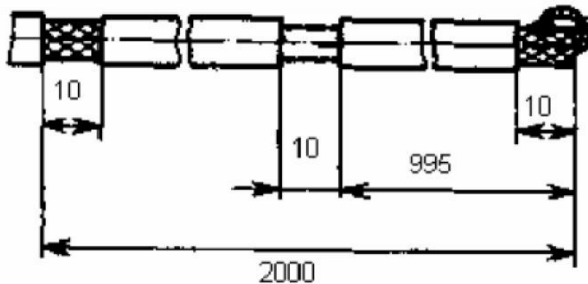
Figure 3 Preparation of the Coupling Loop for the UA6AGW Antenna for the 40-m Band (Dimensions in mm)
