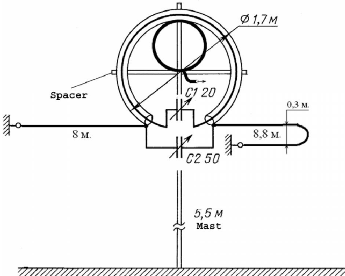
Figure 1 UA6AGW Antenna V.40.20
