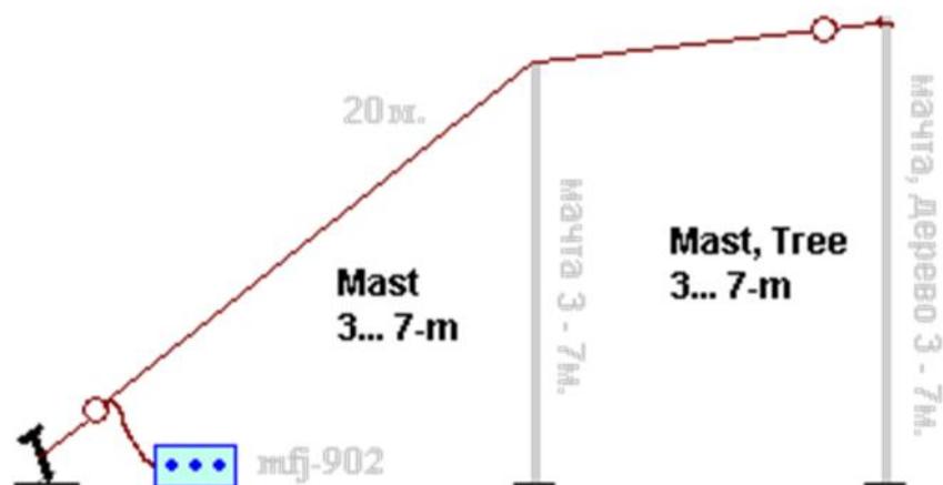
Figure 2 Expedition Sloper Antenna in 20- meters length
