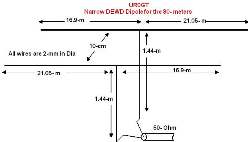
Figure 1 Design of the Super Narrow DEWD Dipole Antenna for the 80- meters with a Stub Matching
