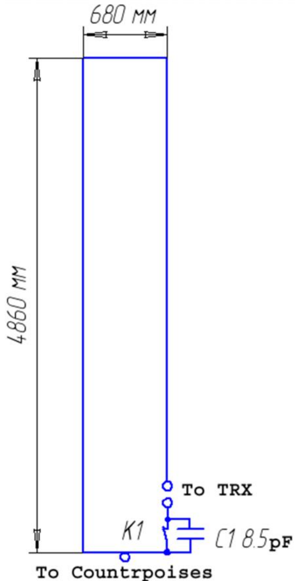
Figure 1 Vertical Stub Antenna for 40 and 20-meter Bands
