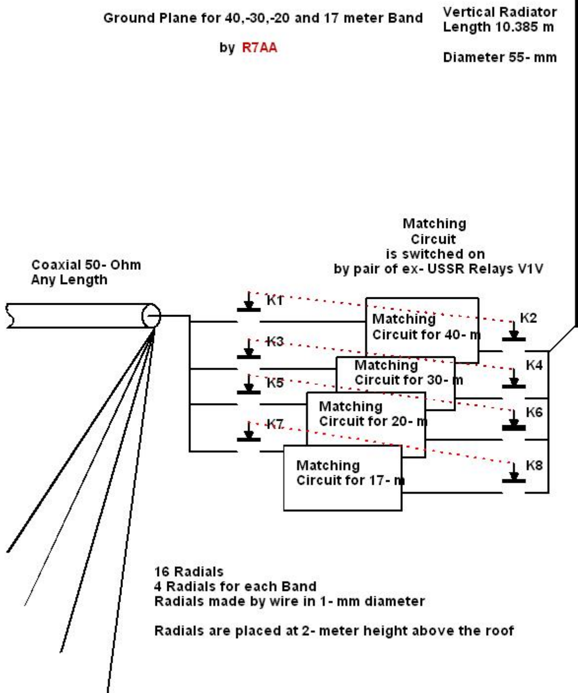
Figure 1 Ground Plane for the 40,- 30,- 20 and 17- meter Bands
