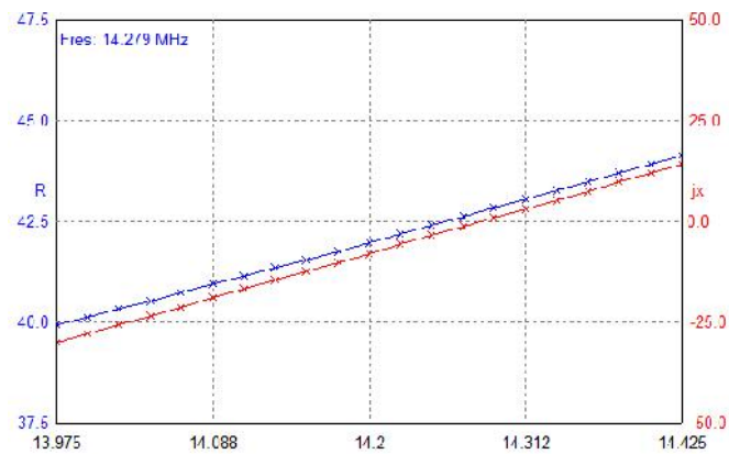
Figure 5 Input Impedance of the Simple Folded Dipole Antenna in Free Space
