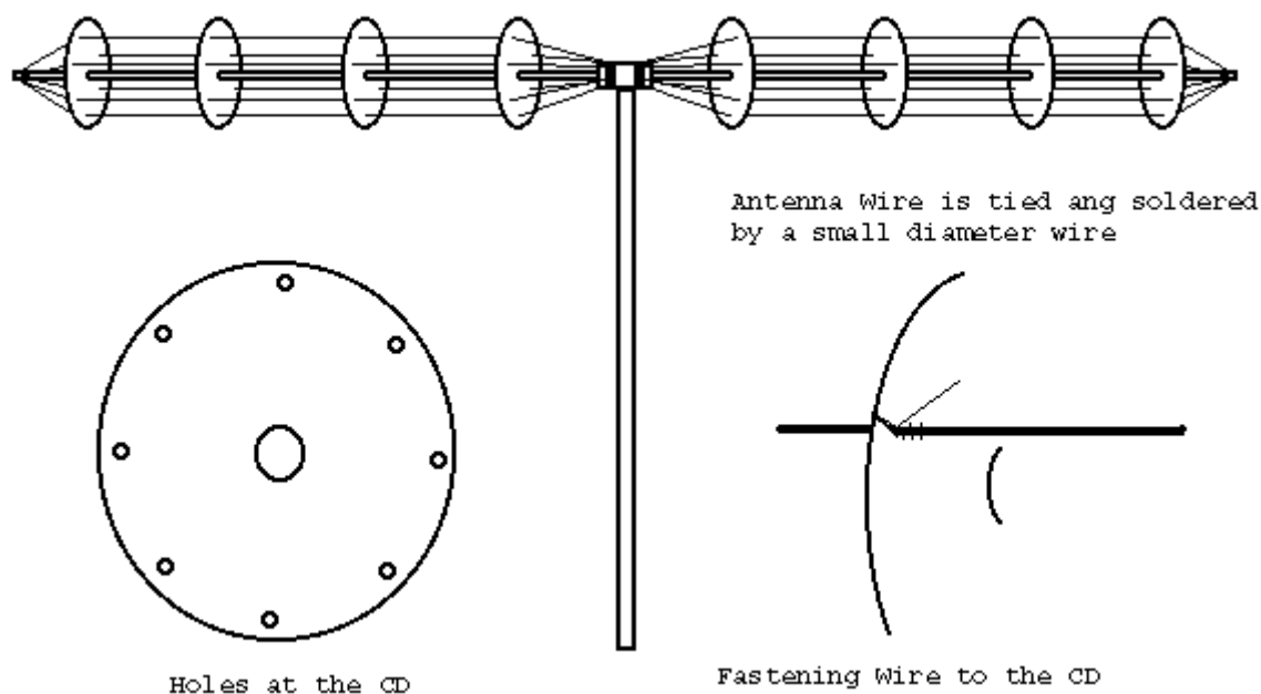
Figure 1 CD Antenna
