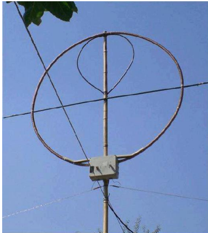
Figure 4 Picture of the UA6AGW Antenna for the 40-m Band
