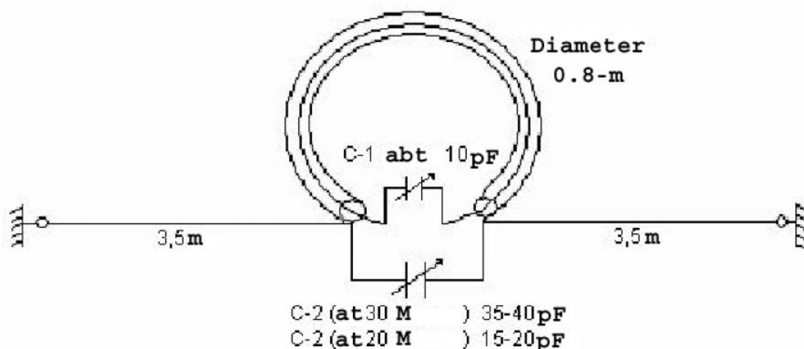
Figure 1 UA6AGW Antenna
