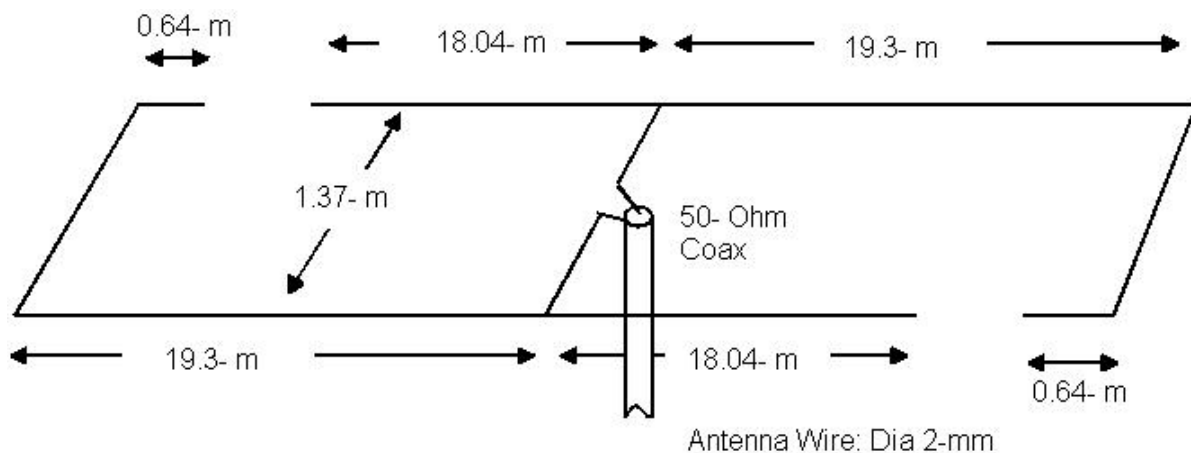
Figure 2 Shortened DEWD Dipole Antenna for the 80- meters
