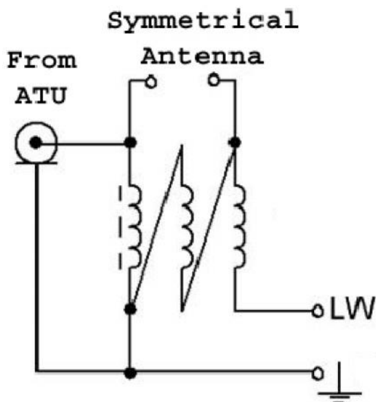
Figure 3 Broadband Transformer
