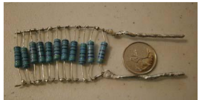
Figure 2 Practical Design of Home- Brew Termination Resistor
