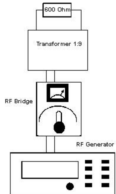
Figure 3 Circuit for Testing of a Working Range of the RF Transformer
