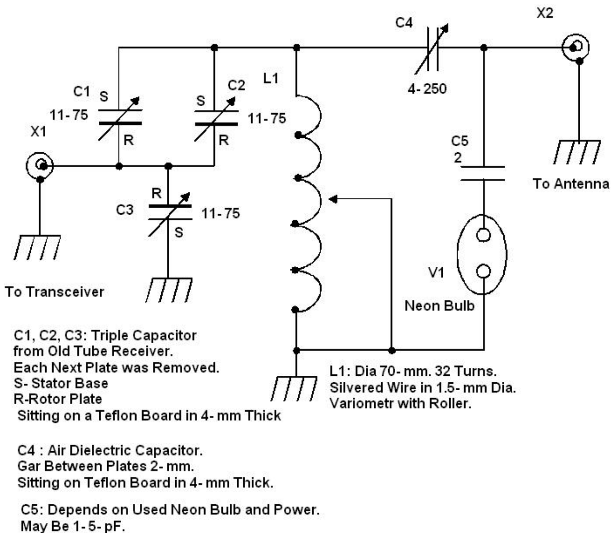
Figure 4 Antenna Tuner by RX3MS for his Helical Antennas
