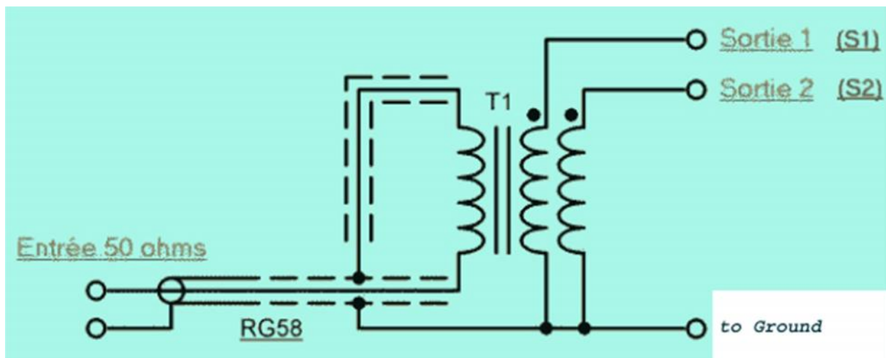
Figure 5 ATU of the UR5WCA Balcony Antenna
