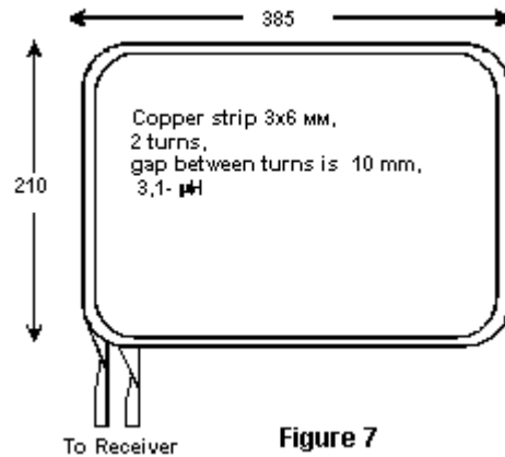
Figure 7 SW Magnetic Loop antenna
