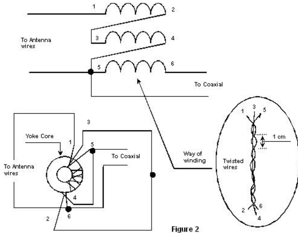
Figure 2 Transformer 9:1
