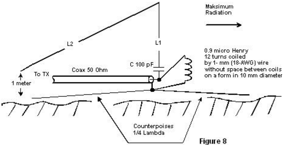
Figure 8 Matching Device of the Field Antenna for the 40- meters
