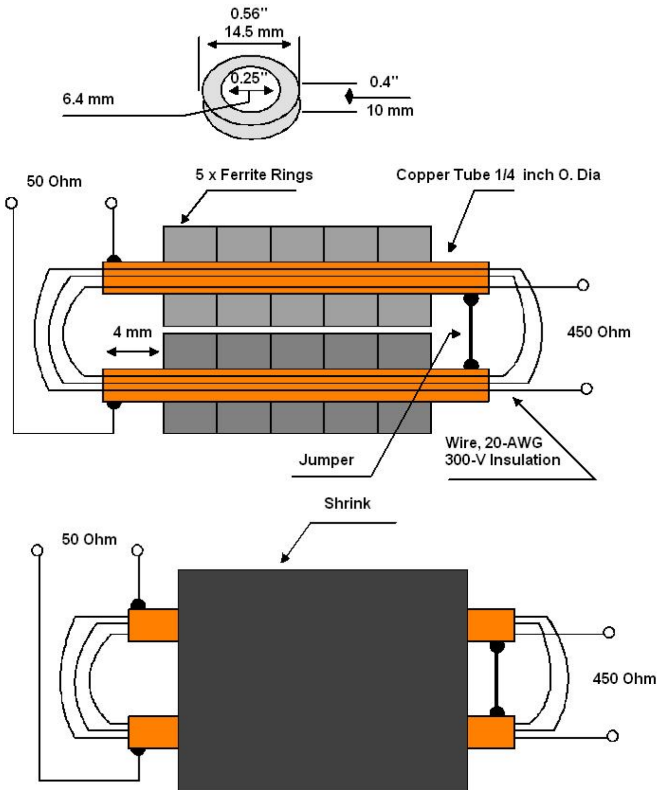
Figure 1 Transformer with Insulated Windings
