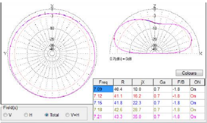
Figure 4 DD of the L-Vertical Antenna for the 40-meter Band
