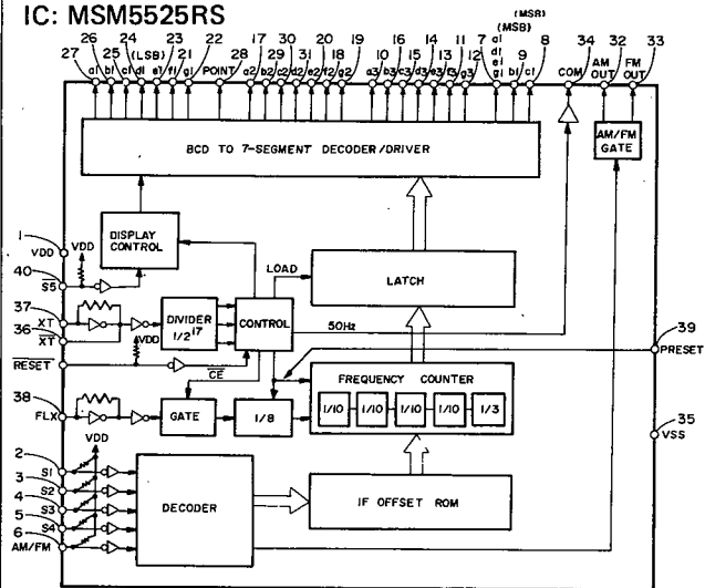
IC: MSM5525RS
