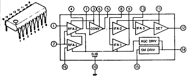
IC: LA1240
