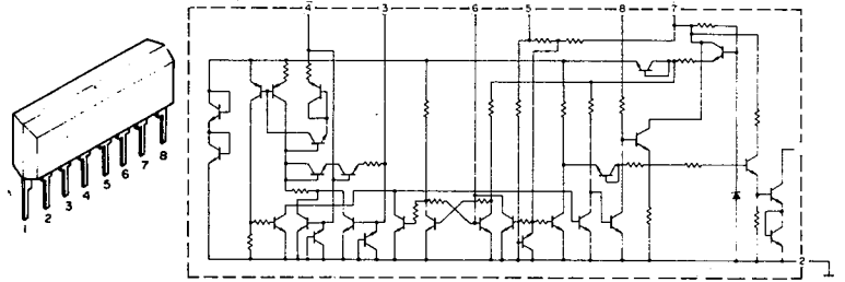
IC: HA12002
