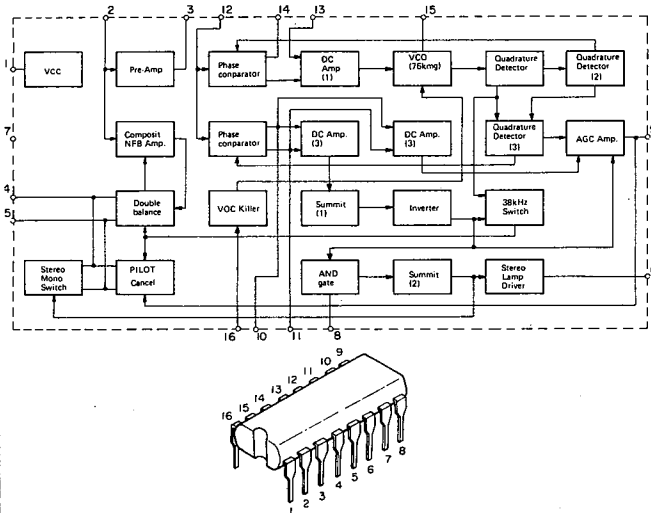
IC: KB4437
