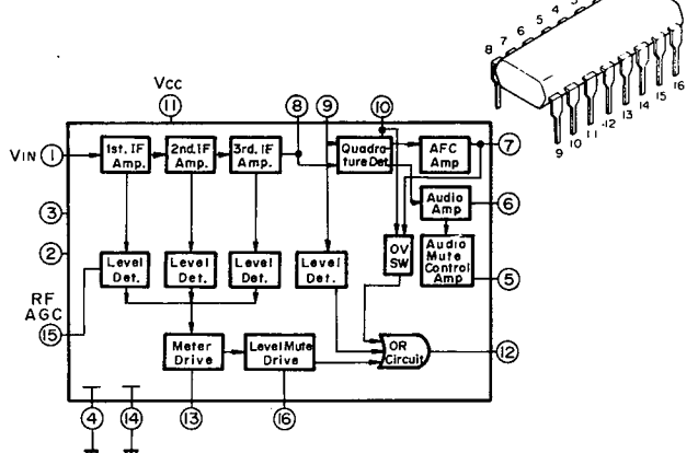
IC: LA1240
