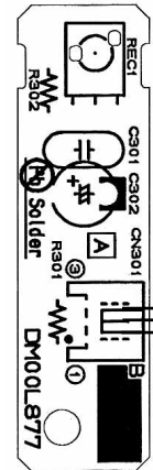
Receiver P.C. board.
