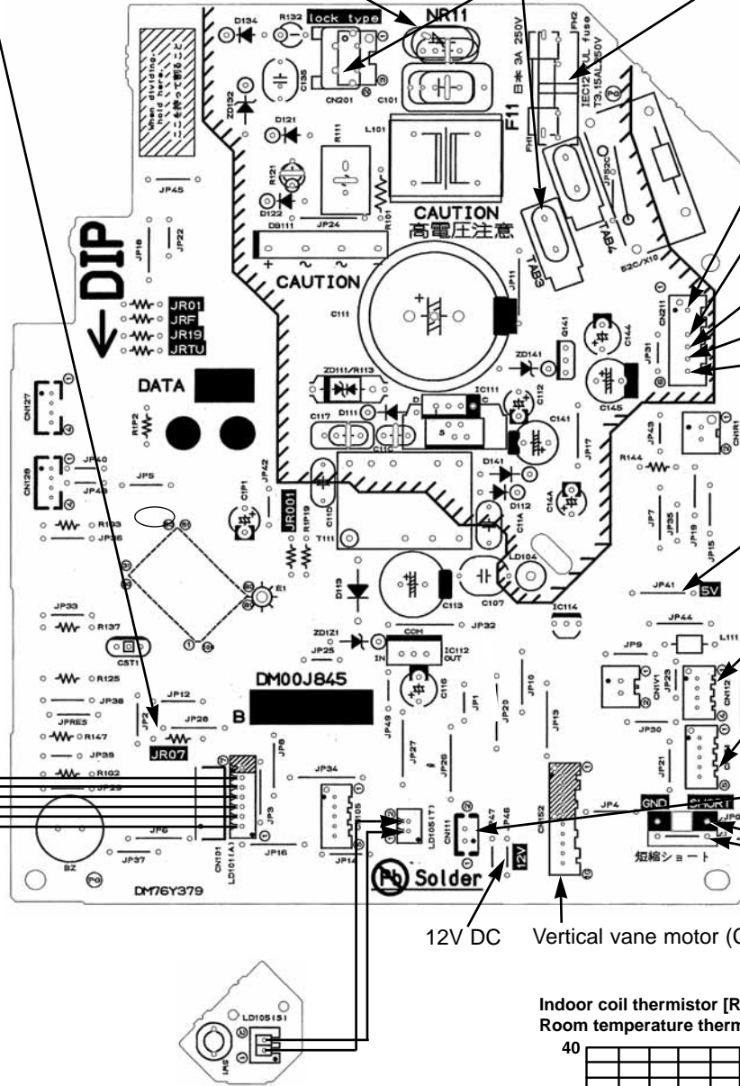
SW P.C. board
