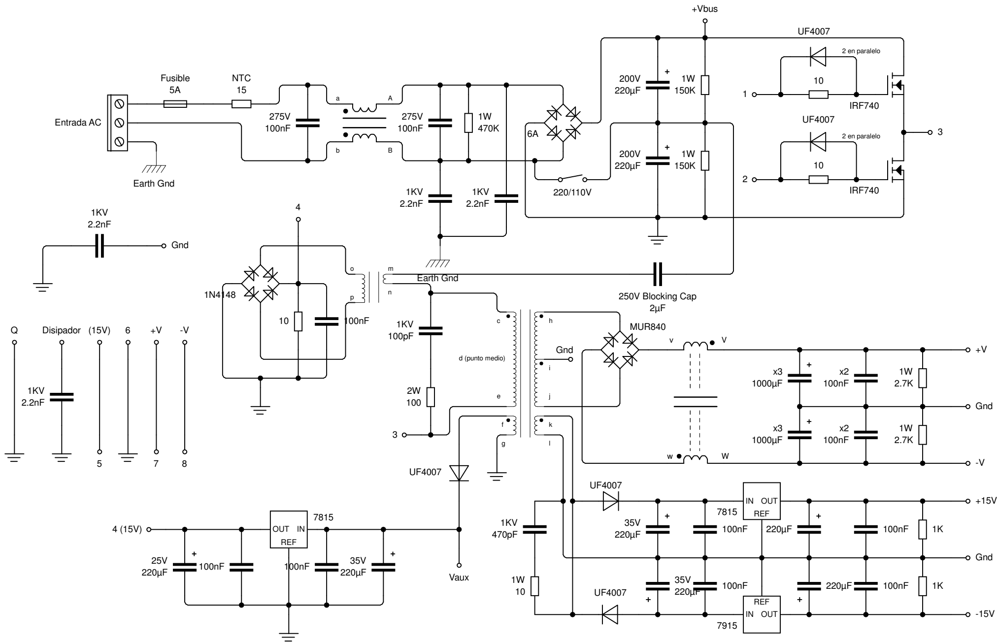
SMPS Half-Bridge 800W 1.0 - Esquema
