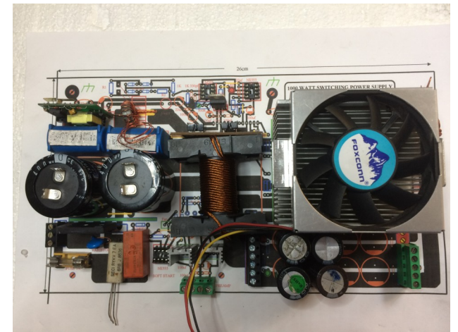
Basic arrangement of components
