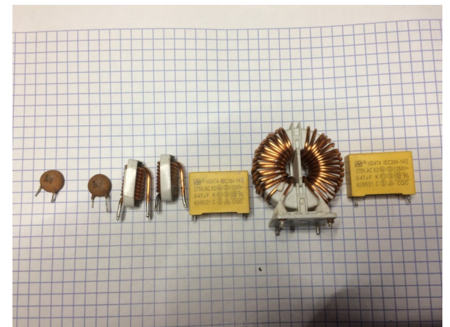
EMI filter parts to be build externally of Main pcb
