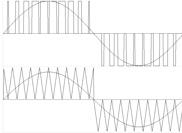
Figure 20: PWM Signal
