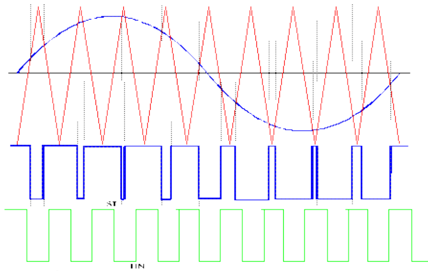
Figure 3: Pulse Width Modulation
